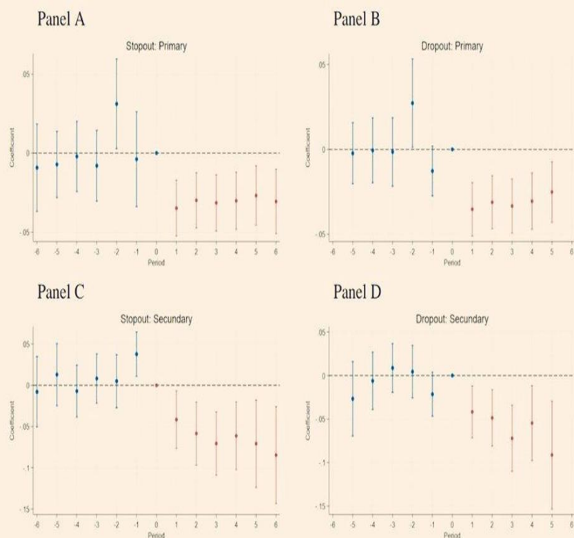
Figure - A 1. Parallel trends event study – Subsample
